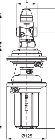
AVPQ 4 (PN25) DN 15 - 50 \Delta p = 0.2 - 1.0 \Delta p = 0.3 - 2.0
