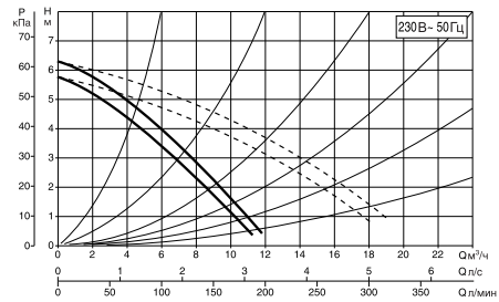
ДРН 120/250.40 Т
