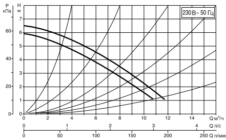
ВРН 120/250.40 Т
