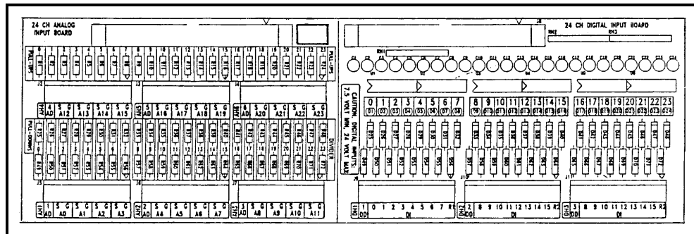
Figure 6, ADI Board
