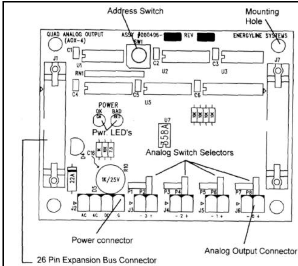
Figure 7, AOX Board
