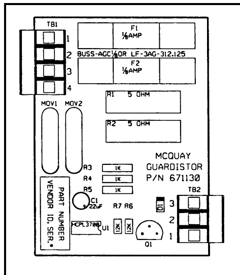
Figure 9, Guardistor Board
