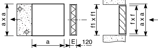
VAF arrangement - The filter box E allows filter removal from one of the four sides.
