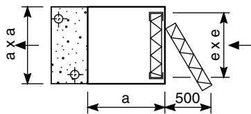
VAL arrangement - Filter removal
