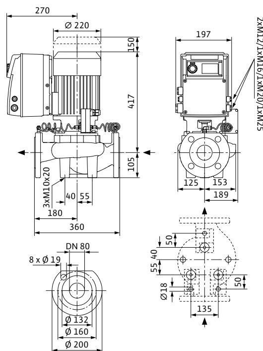
ВeroLine-IP-E 80/140-4/2
