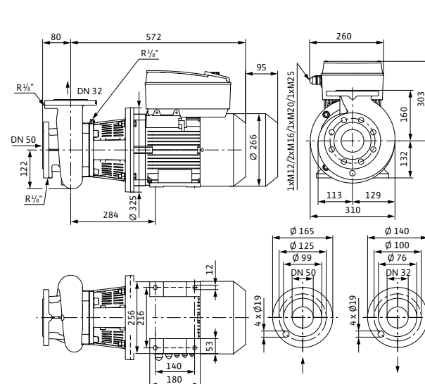
CronoBloc-BL-E 32/170-5,5/2-R1
