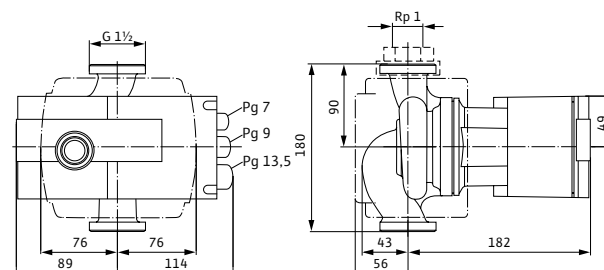
Stratos 25/1-8
