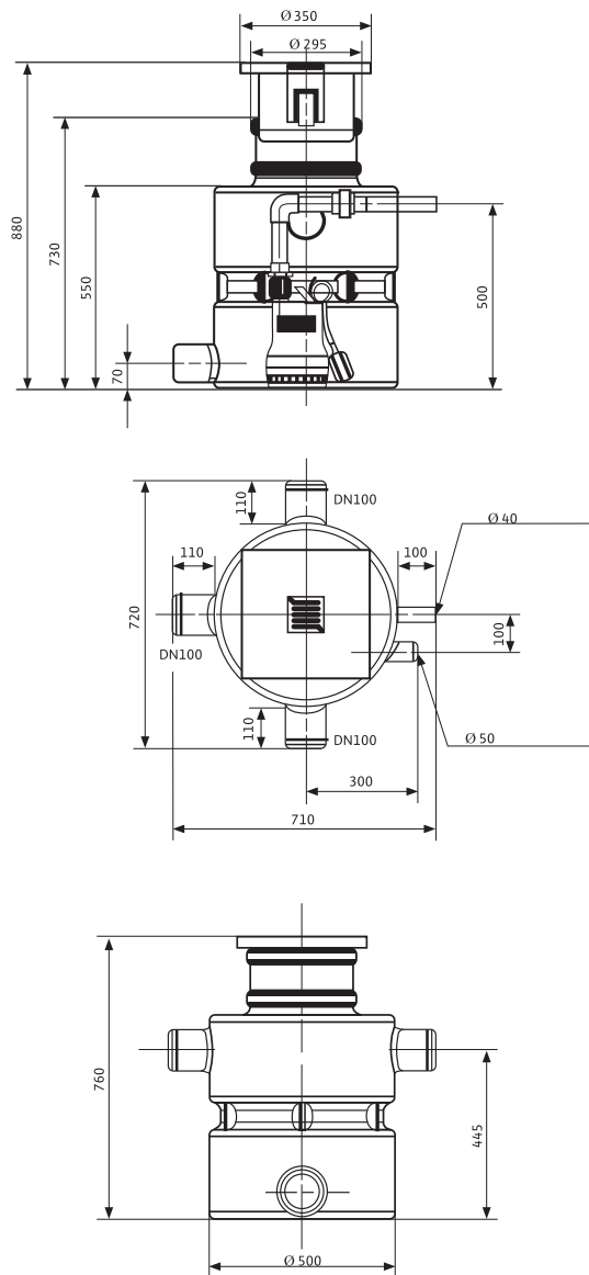
Wilo-DrainLift Box 32
