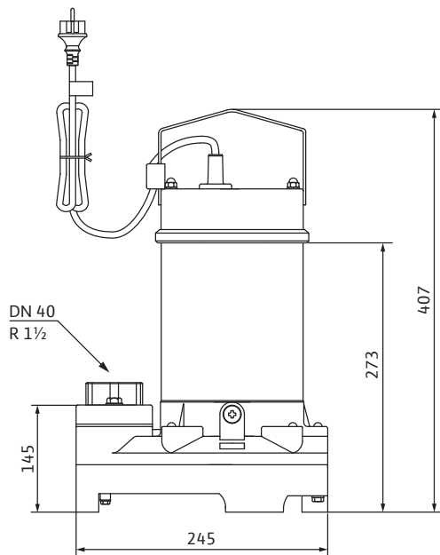
Wilo-Drain TS 40/10
