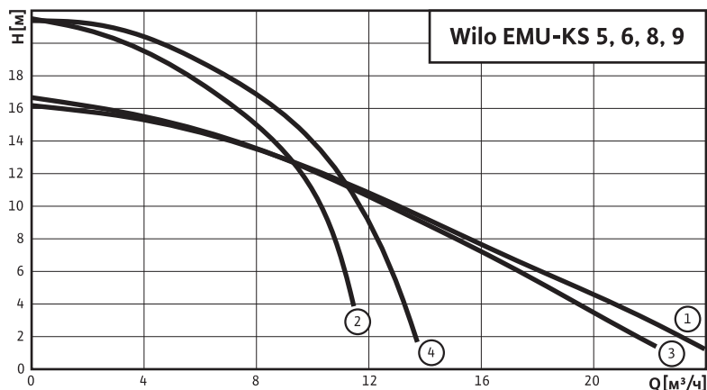
Wilo-EMU KS 5, 6
