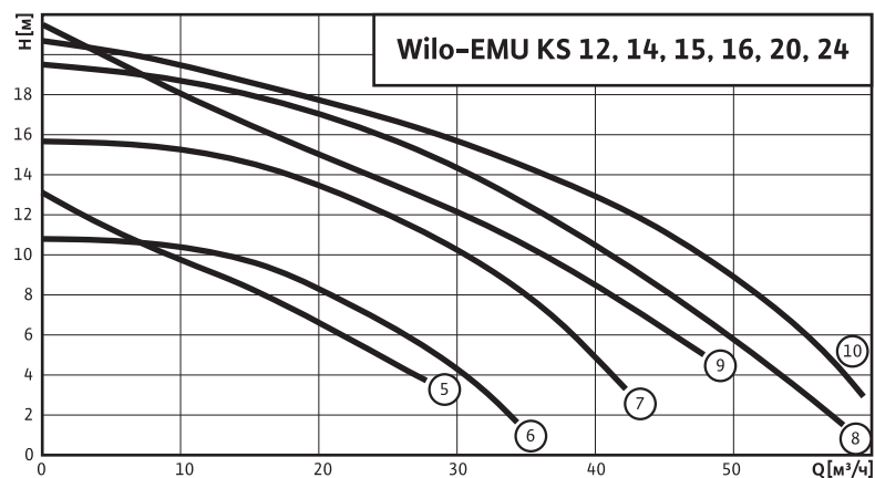
Wilo-EMU KS 12
