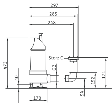
Wilo-EMU KS 20
