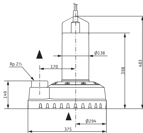
Wilo-Drain TS 65 H 117/22
