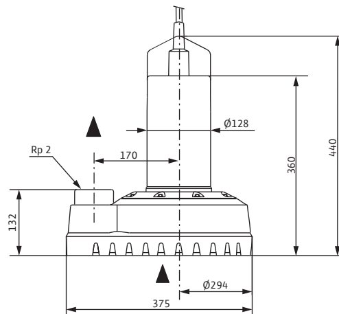
Wilo-Drain TS 50 H 122/15
