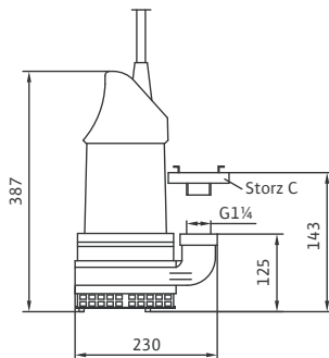
Wilo-EMU KS 8, 9
