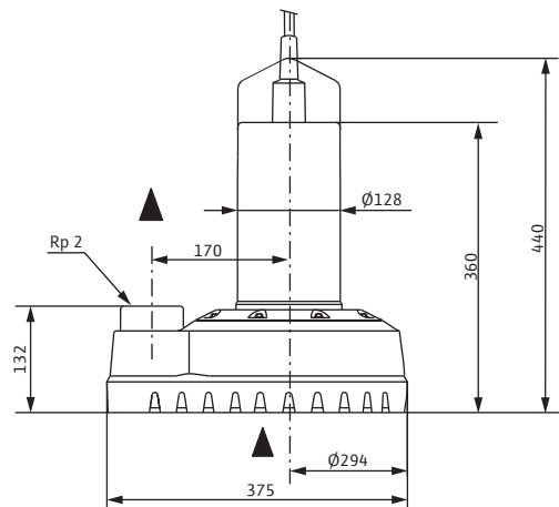
Wilo-Drain TS 50 H 111/11
