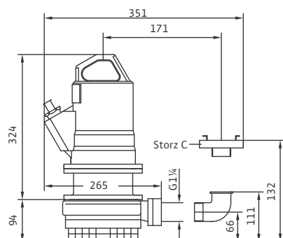
Wilo-EMU KS 5, 6
