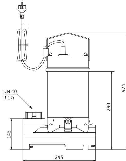
Wilo-Drain TS 40/14
