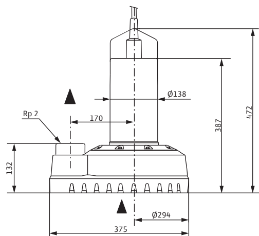
Wilo-Drain TS 50 H 133/22
