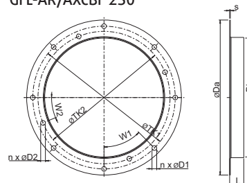
GFL-AR/AXCBF 250
