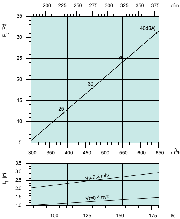
VVKN-B - 600
