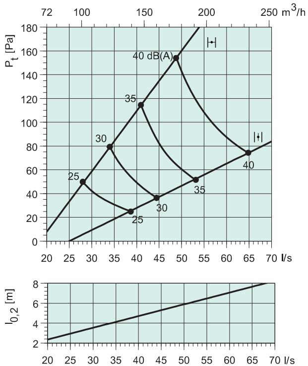
Sinus-BR-125
