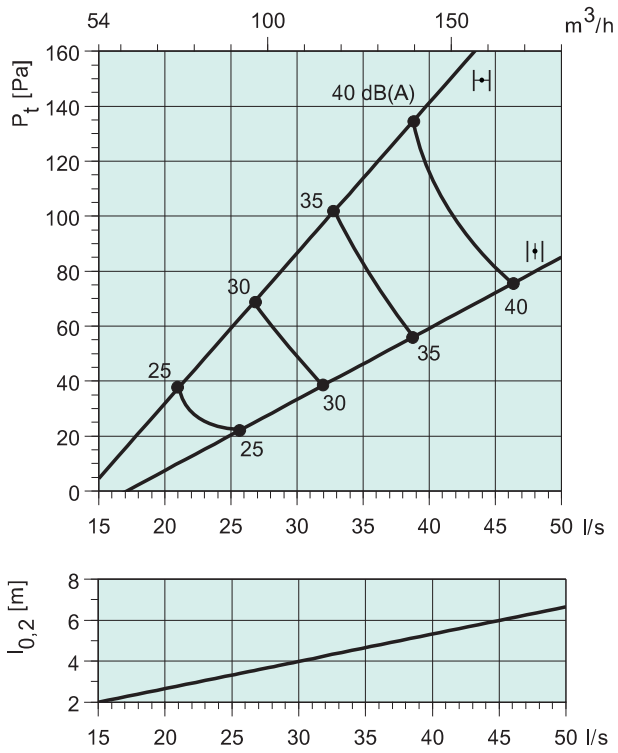
Sinus-BR-100
