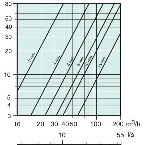
Pa VTK 160
