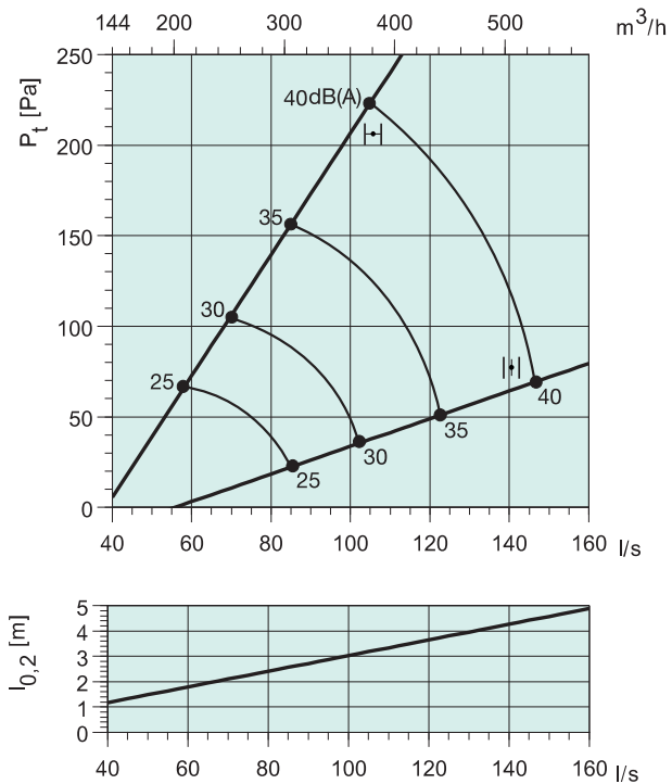
TSK 250 + THOR 200-250
