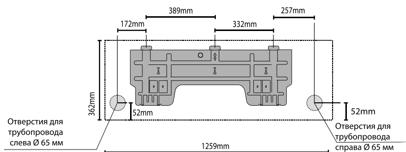
SYSPLIT WALL SMART V3 30-36 HP Q
