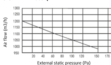
SYSVRF HRV 1000 Q
