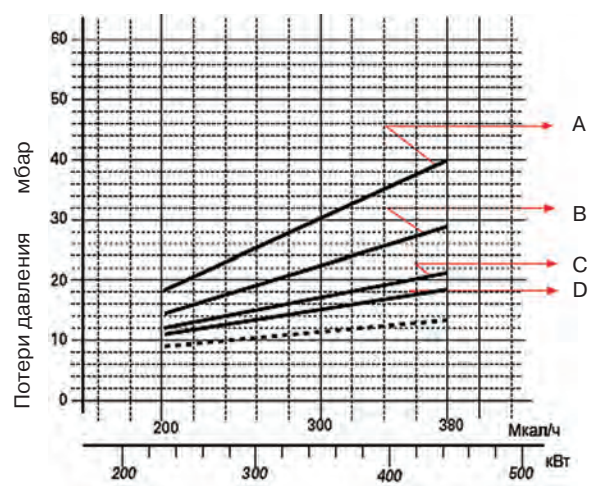
RLS 38
