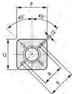
FS15D - FS20D
