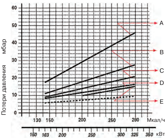
RLS 28
