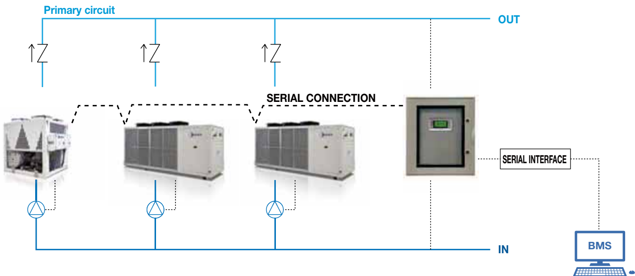
Simplified example of a 2-pipe system with two heat pumps and one chiller managed by KMTM/SI. The system provides for summer operation with the two heat pumps and the chiller operating in SUMMER mode and winter operation with the inversion of the heat pumps and the shutdown of the chiller.
