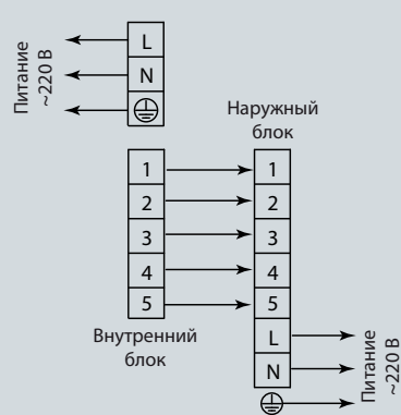
QV-I24FA/QN-I24UA
