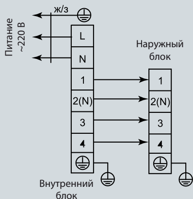
QV-I18DA/QN-I18UA
