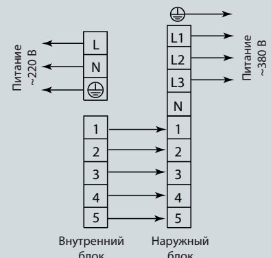
QV-I48_60FA/QN-I48_60UA
