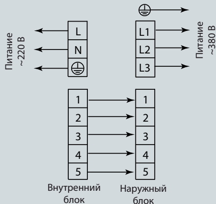
QV-I36DA/QN-I36UA
