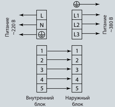
QV-I36FA/QN-I36UA
