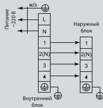
QV-I18FA/QN-I18UA
