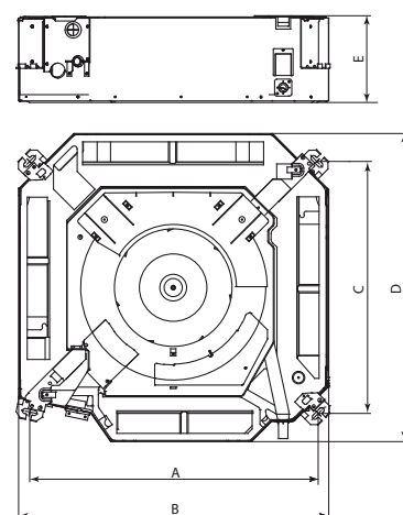
QV-I24_36_48_60CA
