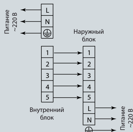
QV-I24DA/QN-I24UA
