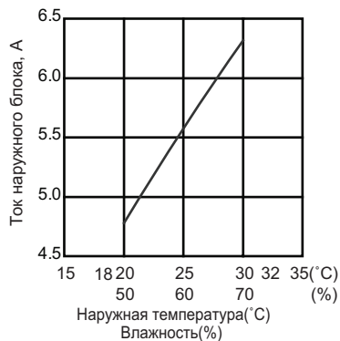
MUZ-GE50VA
