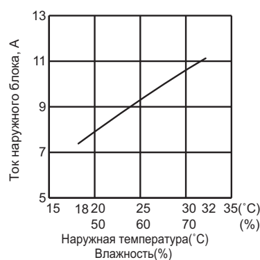
MUZ-GA71VA
