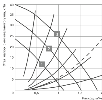
STM-H 60-4,0-C24-F
