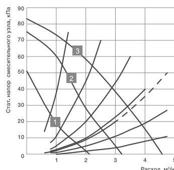
STM-H 80-10,0-C24-F
