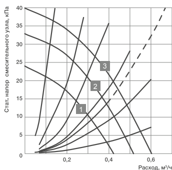
STM-H 40-1,6-C24-F
