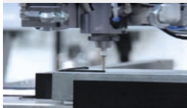
Robot for fitting bi-component form-in-place gasket
