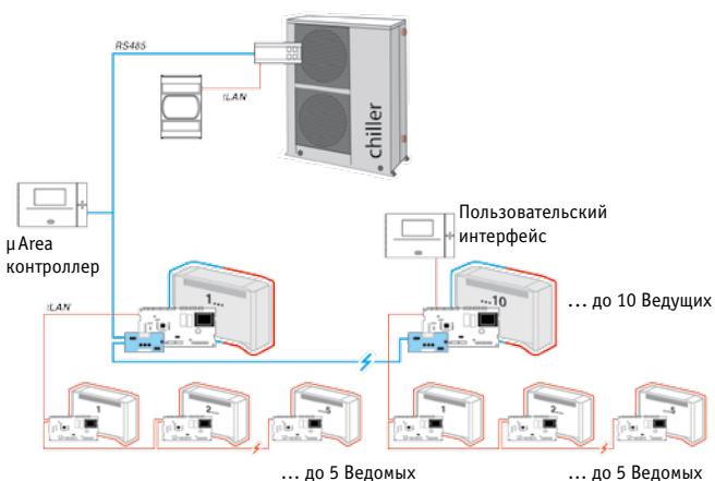
μe-dronic
