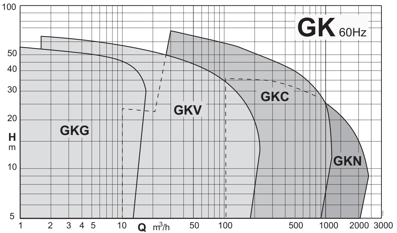
Submersible pumps
