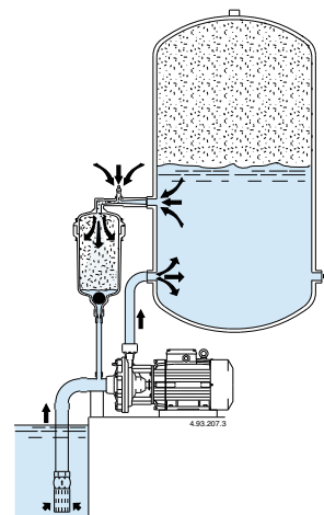
3) The water level in the ARIAMAT drops until the ball valve moves to the bottom of the ARIAMAT closing the hole of the pipe connected to the pump. ARIAMAT is now full of water.
