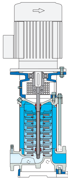
MXV 65, 80
