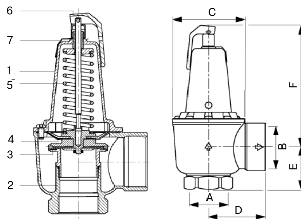
Prescor S 1700, 2"
