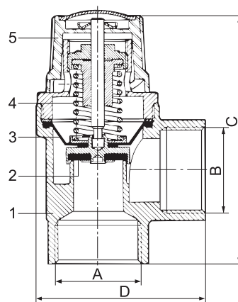
Prescor 3/4"; 1"; 1 1/4"
