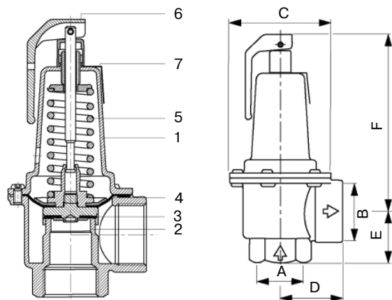
Prescor S 700, 1¼"
