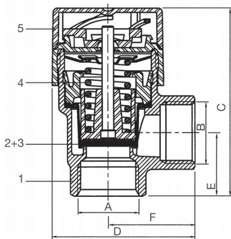
Prescor B 1/2"
