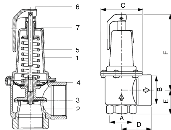
Prescor S 960, 1½"
