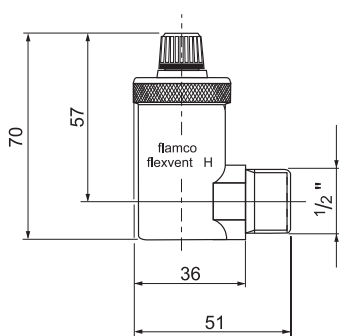
Flexvent H
